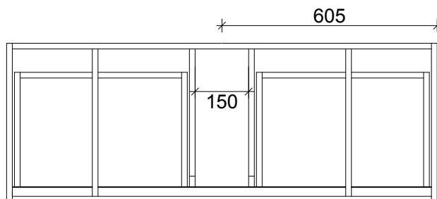
CABINET TOP VIEW
